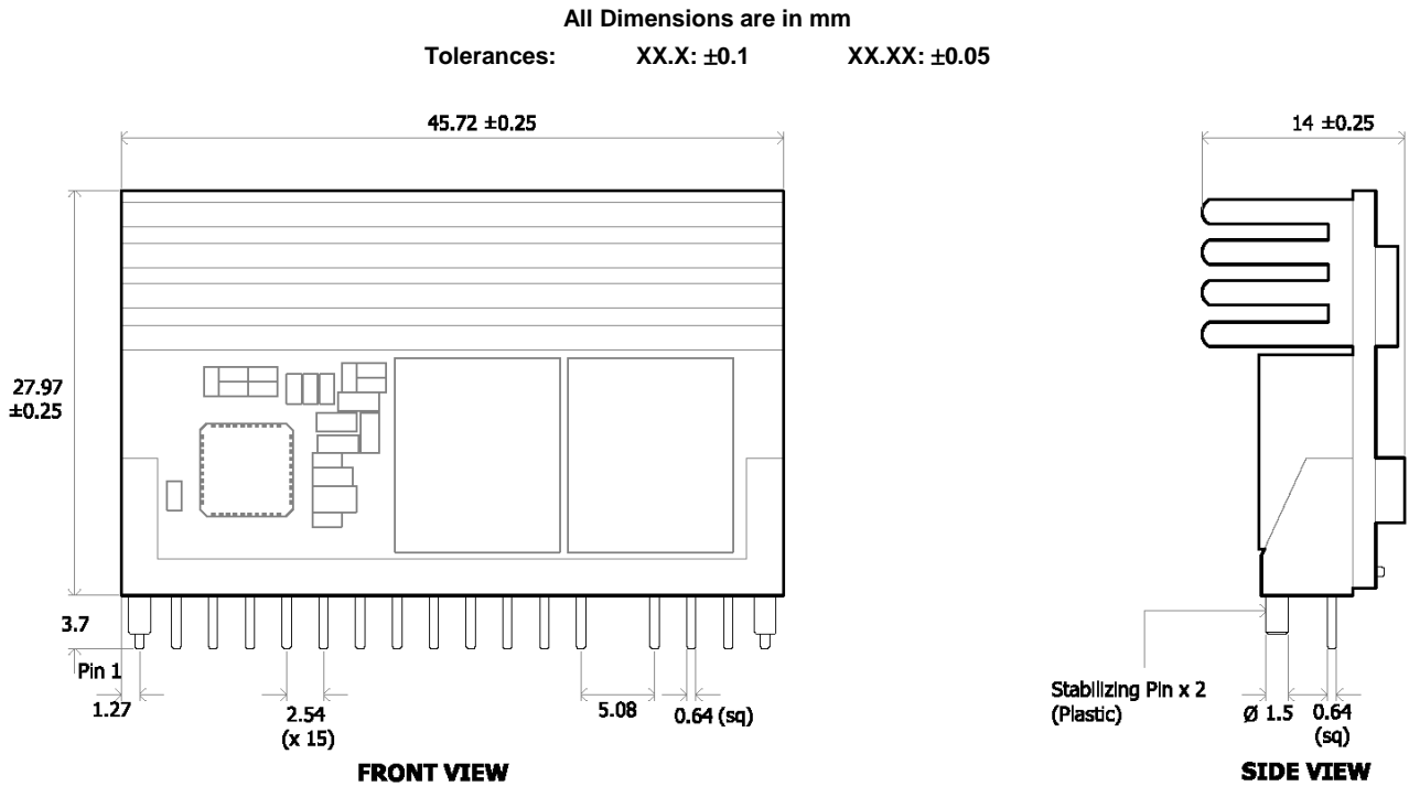
Figure 47. Mechanical Drawing
